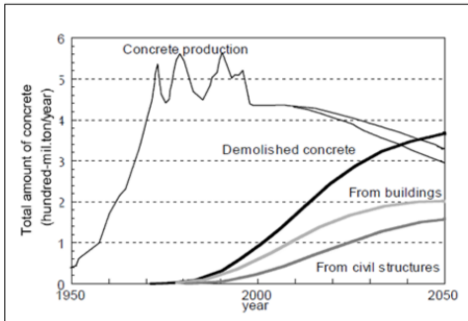
Estimated amount of demolished concrete
