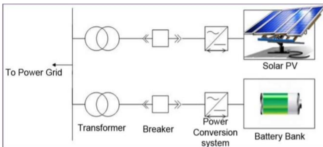
Fig. 2. Simplified one-line diagram of a BESS in parallel with a Solar PV facility connected to the grid on common bus.
