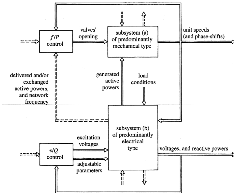
Figure 1.9. Broad block diagram of a generic system.
