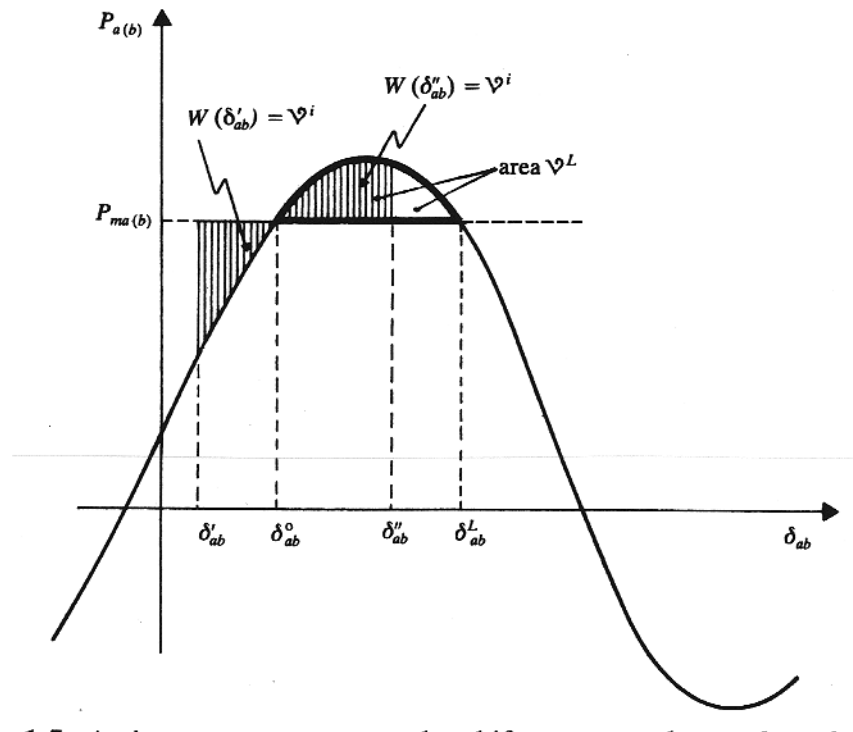
Figure 1.5. Active power versus angular shift curve, used to analyze the relative motion between machines, as in figure 1.2c.
