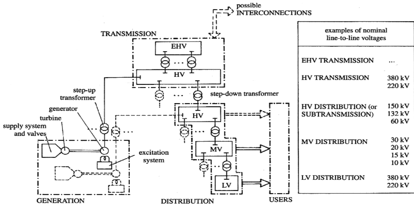
Figure 1.1. Basic elements of an electric power system (EHV, HV, MV, LV mean, respectively, extra-high, high, medium, and low voltage).
