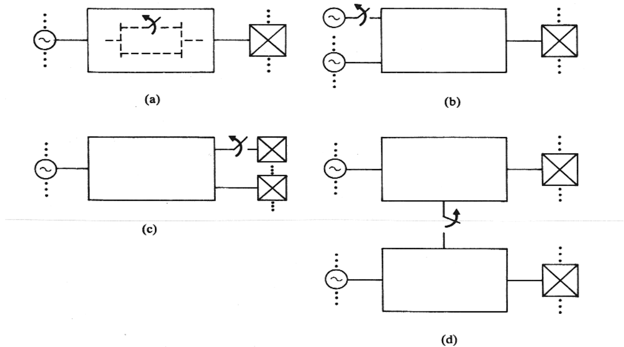
Figure 1.8. Examples of perturbations that permanently alter the system configuration: (a) internal line trip; (b) generating plant outage; (c) loss of a user group; (d) (single) interconnection line trip.
