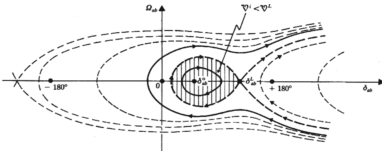
Figure 1.7. Trajectories on the (\delta_{ab}, \Omega_{ab}) plane, for the system of figure 1.2c.
