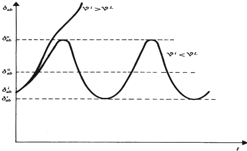
Figure 1.6. Typical behaviors of angular shift between machines for the system of figure 1.2c.
