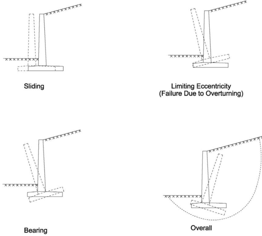
Figure.4-9 External Stability Failure of CIP Semi-Gravity Walls
