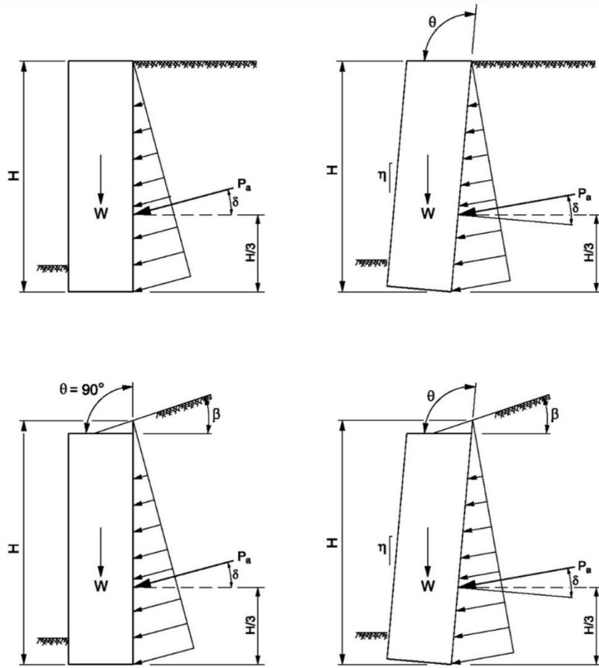
Figure 4-6 Lateral Earth Pressure on Concrete Modular Systems of Constant Width (Source LRFD [Figure 3.11.5.9-1])
