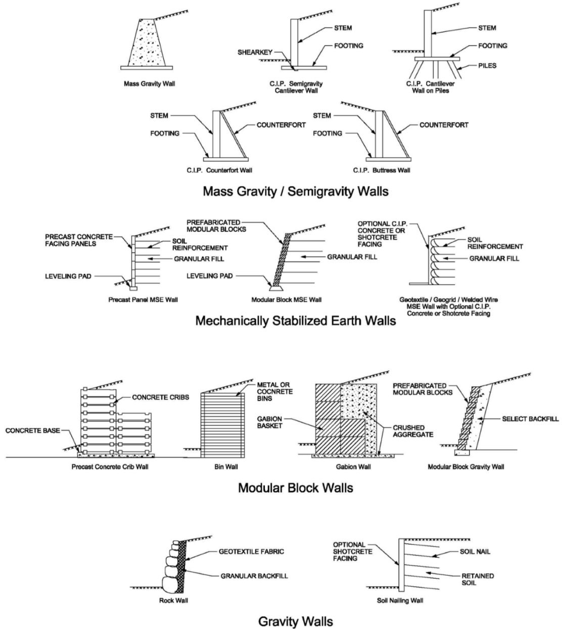
Figure 14.2-1 Gravity Walls
