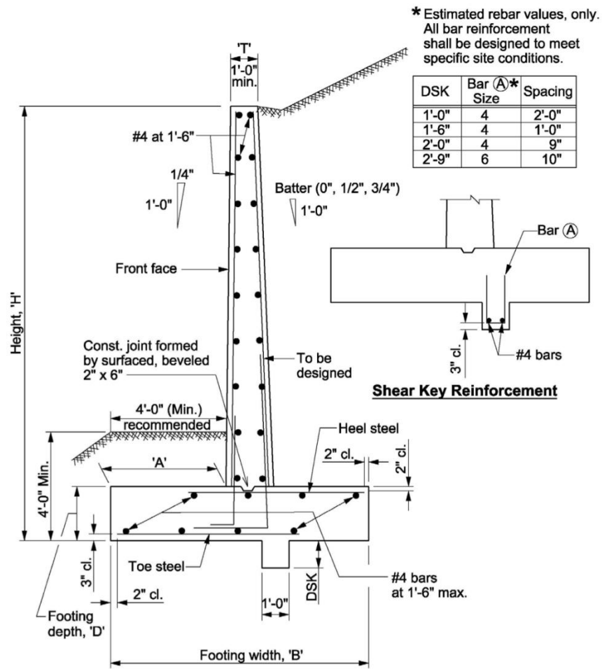
Figure 5-2 CIP Walls General Details
