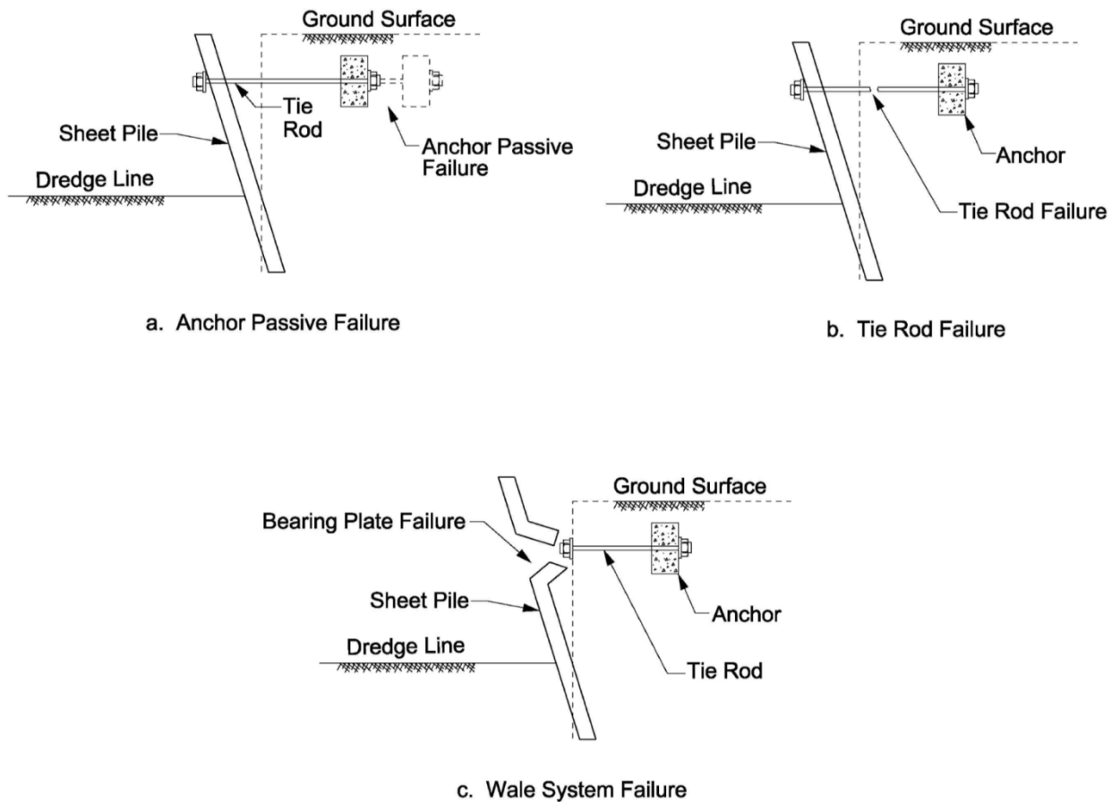
Figure 4-14 Flexural Failure of Non-Gravity Walls
