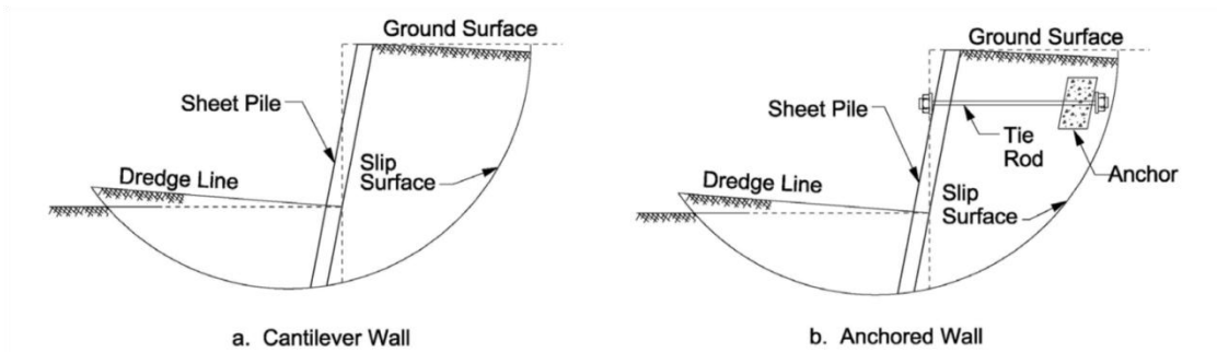
Figure 4-12 Deep Seated Failure of Non-Gravity Walls
