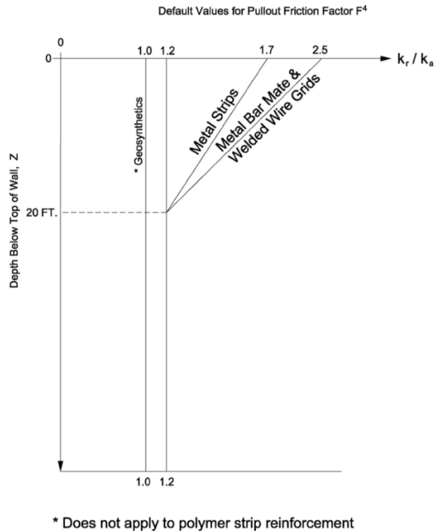
Figure 6-6 Variation of the Coefficient of Lateral Stress Ratio with Depth (Source AASHTO LRFD )
