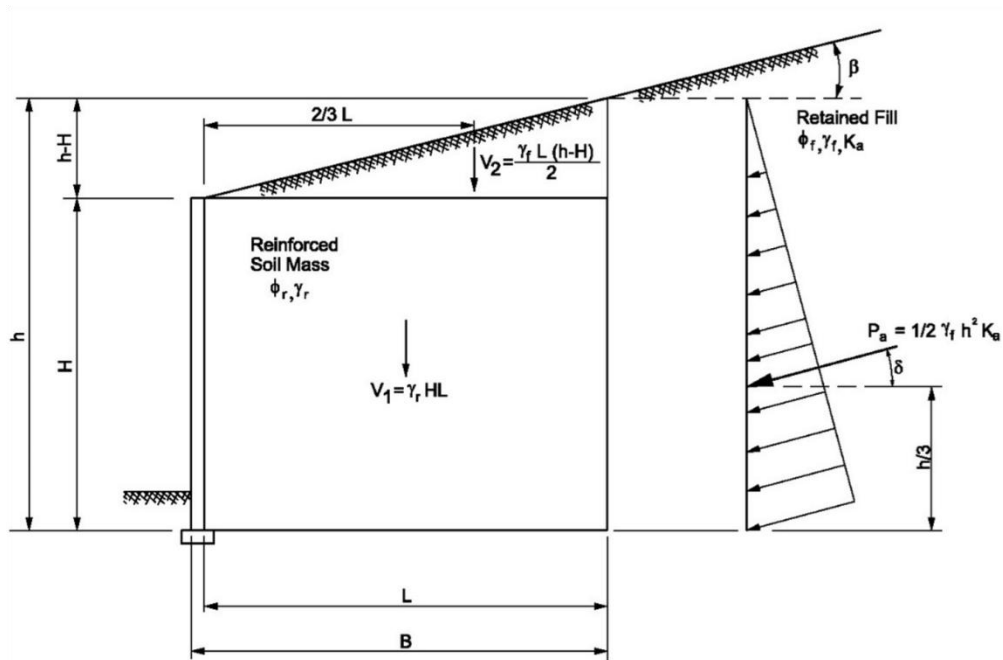
Figure 4-3 MSE Walls Earth Pressure for Sloping Backfill (Source LRFD [Figure 3.11.5.8.1-2])
