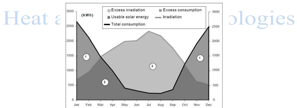
Figure 18: Figure showing an example of the annual variation in solar irradiation and energy consumption for space heating
