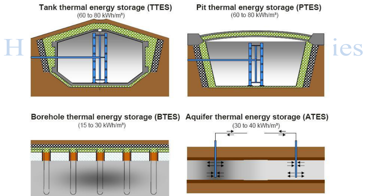
Figure 4: Illustration of seasonal thermal energy storage – concepts (ref. /4/)
