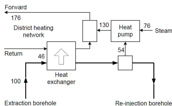
Figure 12: District heating base on geothermal sources (ref. /4/)
