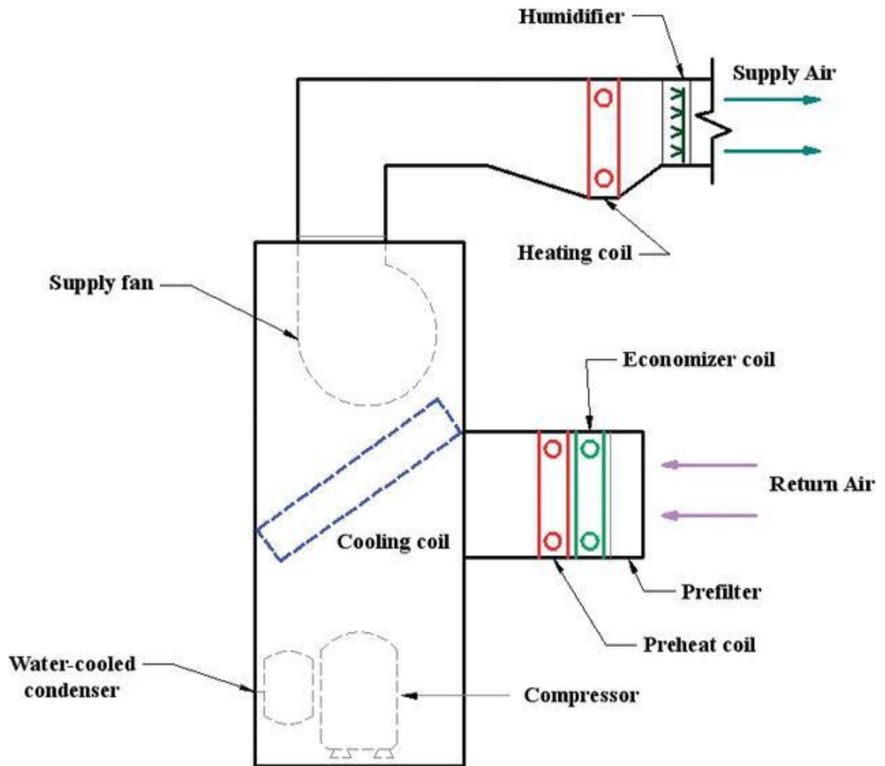
Figure 13. Unitary air-conditioner package.
