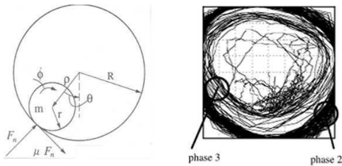
Fig. 10 Left: Variables for describing the touch-down dynamics of the rotor within the stator: rotor speed \Phi , whirl velocity \theta , air gap \rho , mass of the rotor m , normal force F_N and friction force \mu F_N . Right: motion of the rotor center within a circle with the radius of the airgap (0.3 mm). The backward whirl is initiated by a drop down of the rotor, [7].
